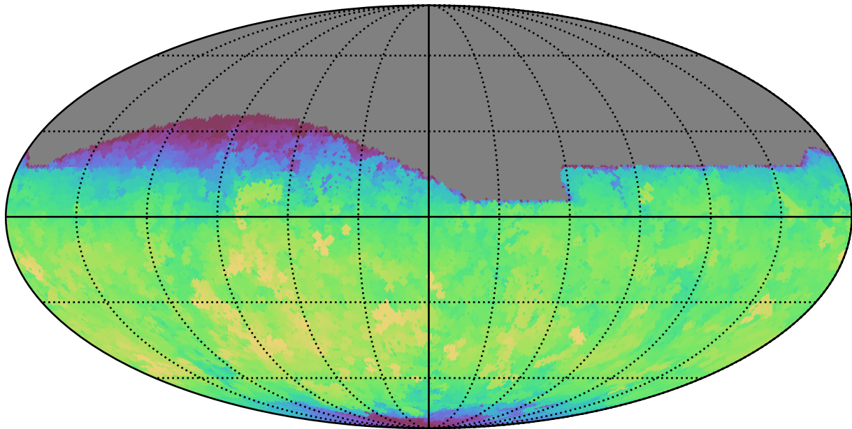
weather_cloudso20v3.4_10yrs All sky r band: Max fiveSigmaDepth
