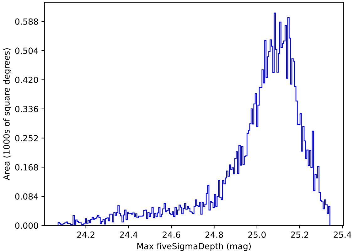
weather_cloudso20v3.4_10yrs All sky all bands: Max fiveSigmaDepth
