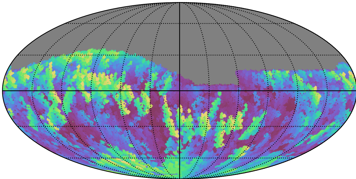
weather_cloudso20v3.4_10yrs Yr 1 z band: Max airmass
