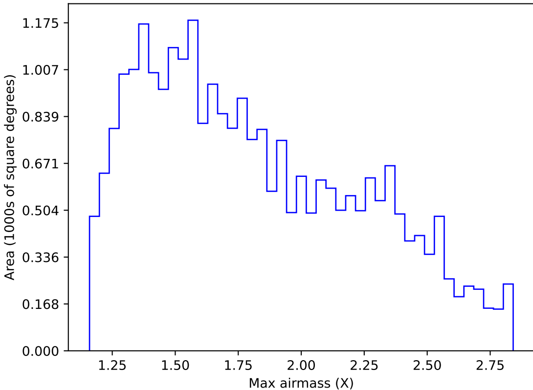
weather_cloudso20v3.4_10yrs Yr 1 z band: Max airmass
