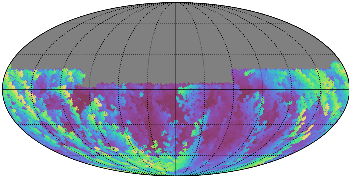
weather_cloudso20v3.4_10yrs Yr 1 y band: Max airmass
