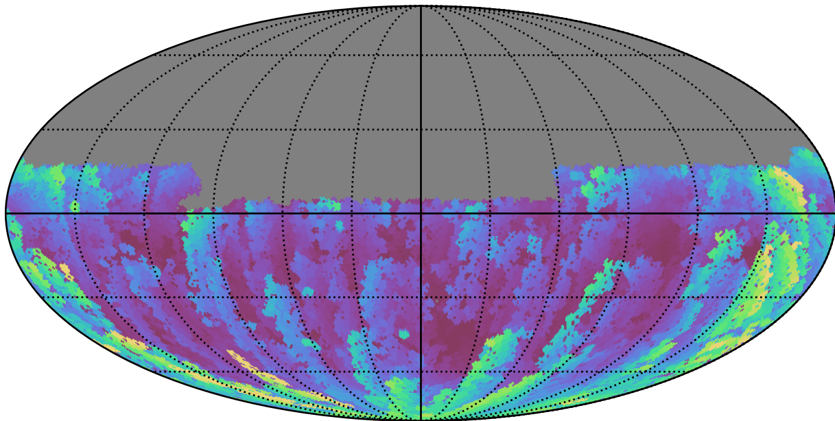
weather_cloudso20v3.4_10yrs Yr 1 u band: Max airmass
