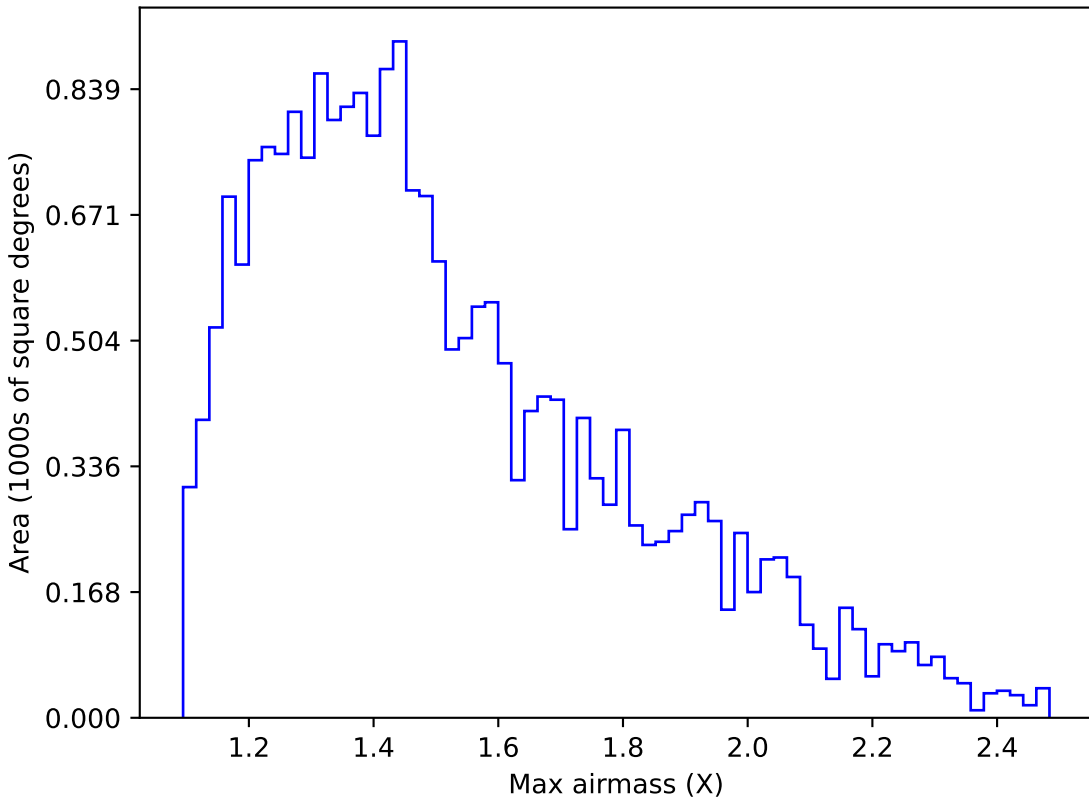
weather_cloudso20v3.4_10yrs Yr 1 u band: Max airmass
