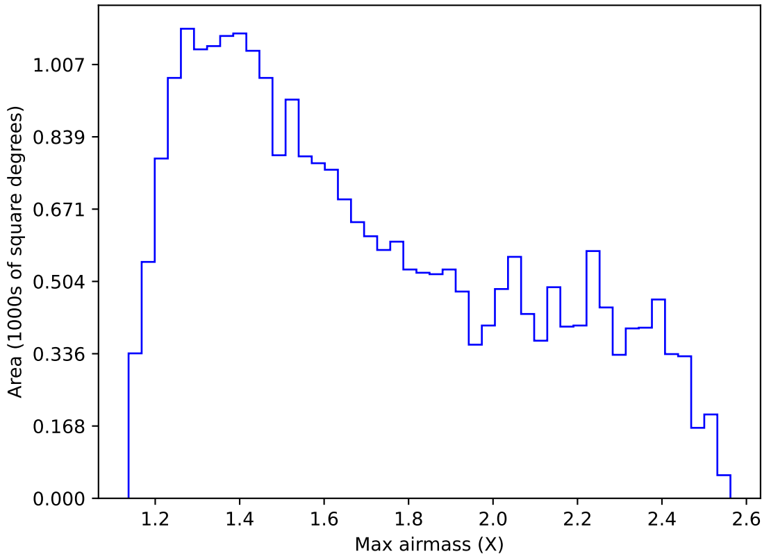
weather_cloudso20v3.4_10yrs Yr 1 r band: Max airmass
