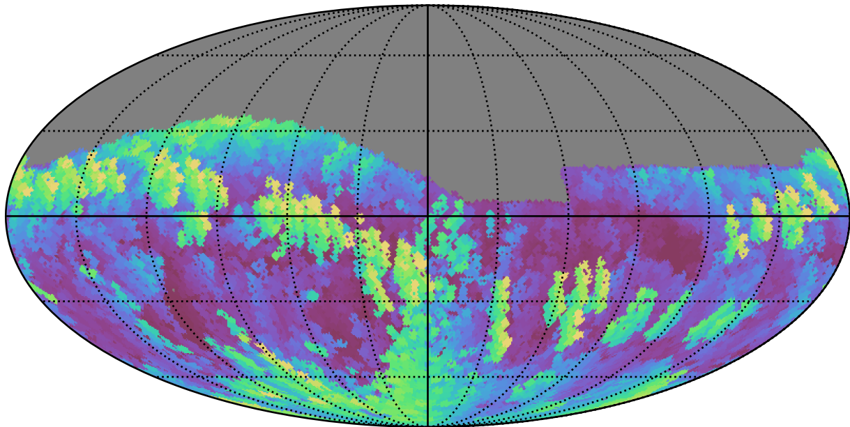
weather_cloudso20v3.4_10yrs Yr 1 i band: Max airmass
