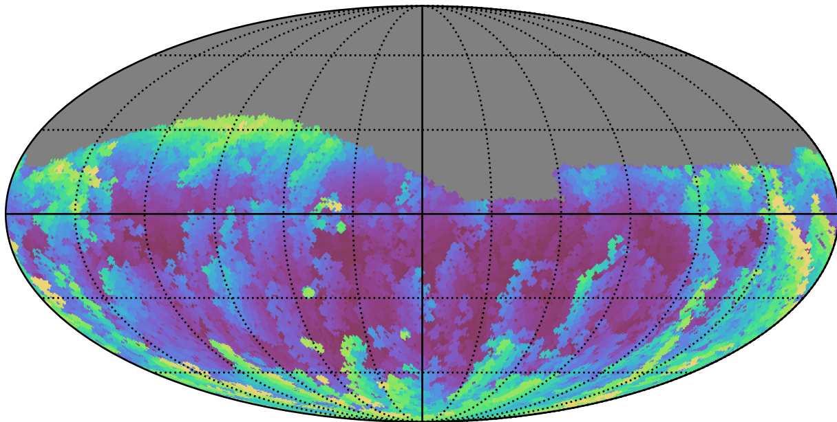
weather_cloudso20v3.4_10yrs Yr 1 g band: Max airmass
