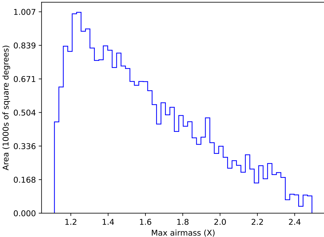
weather_cloudso20v3.4_10yrs Yr 1 g band: Max airmass
