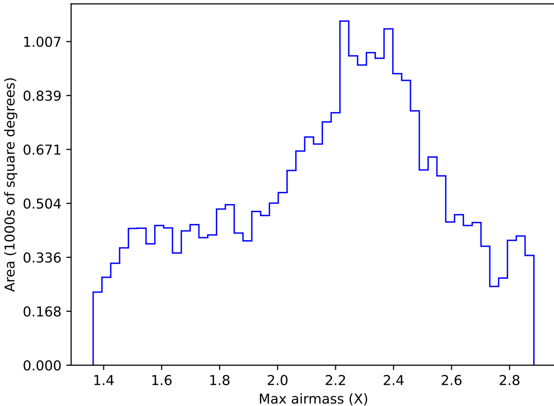
weather_cloudso20v3.4_10yrs Yr 1 all bands: Max airmass
