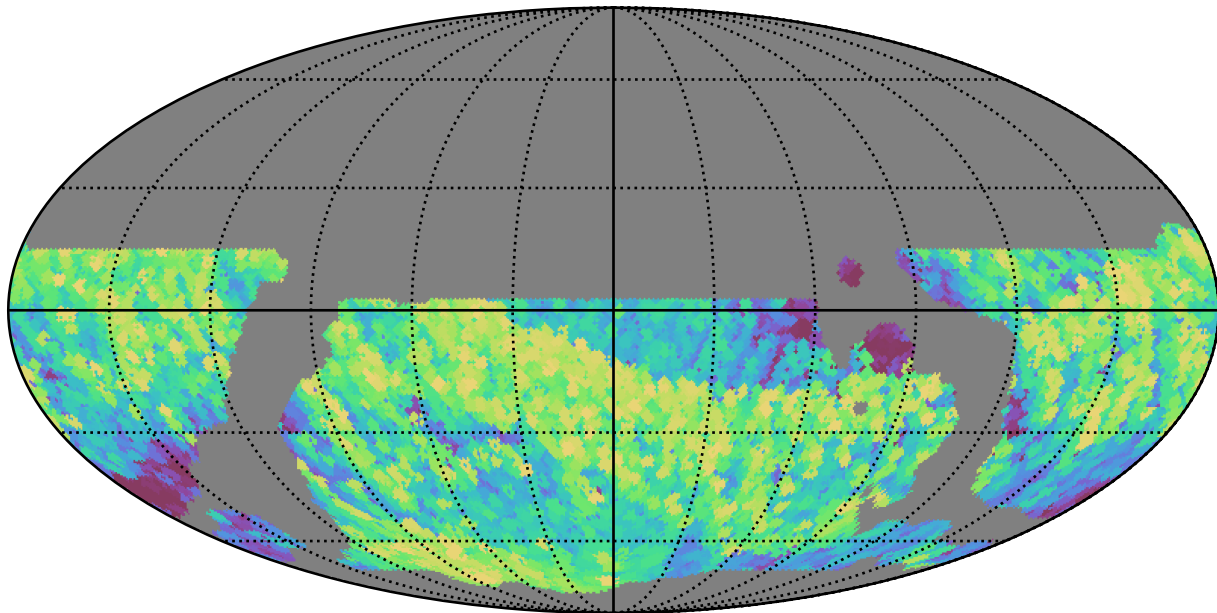
weather_cloudso20v3.4_10yrs WFD z band: Max airmass
