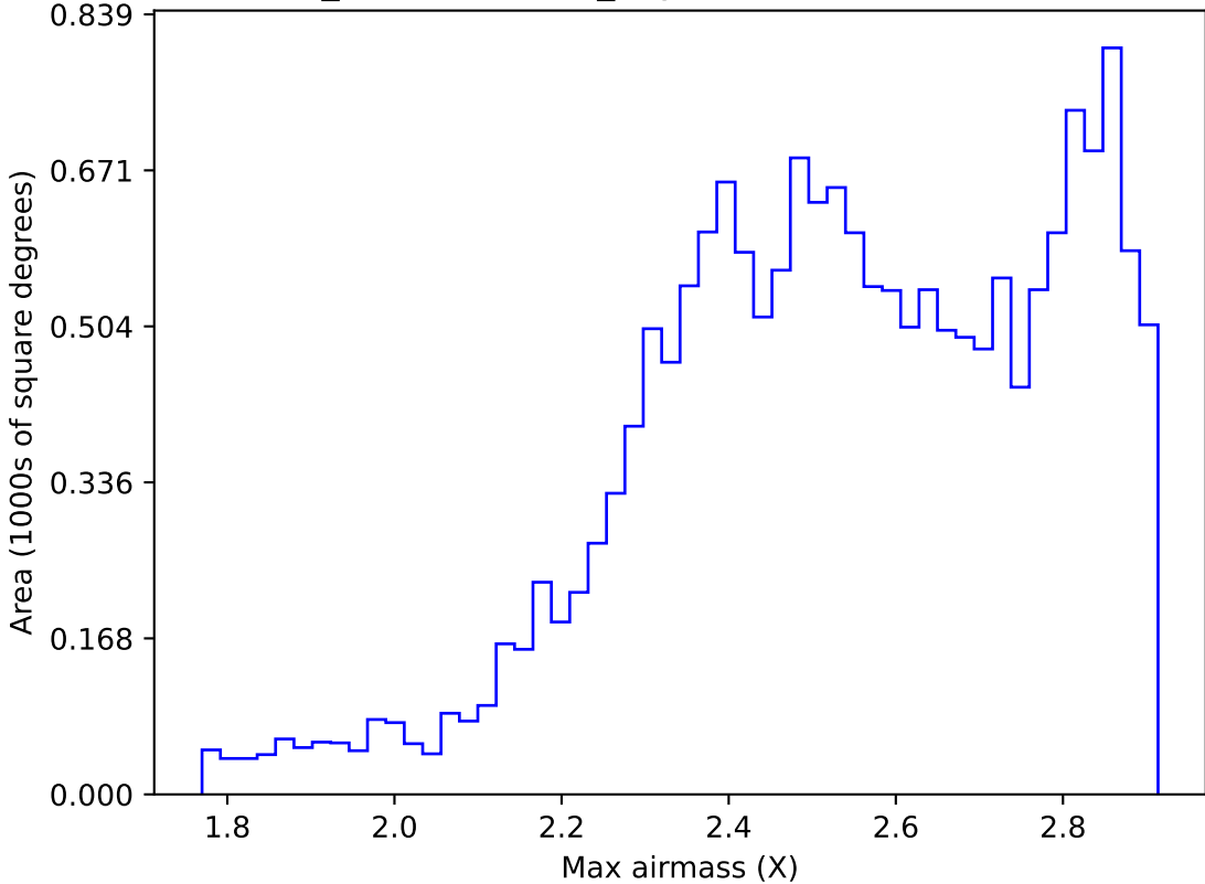
weather_cloudso20v3.4_10yrs WFD z band: Max airmass
