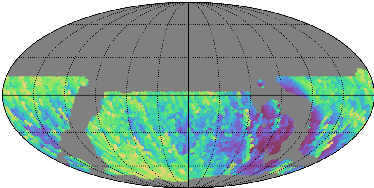
weather_cloudso20v3.4_10yrs WFD y band: Max airmass
