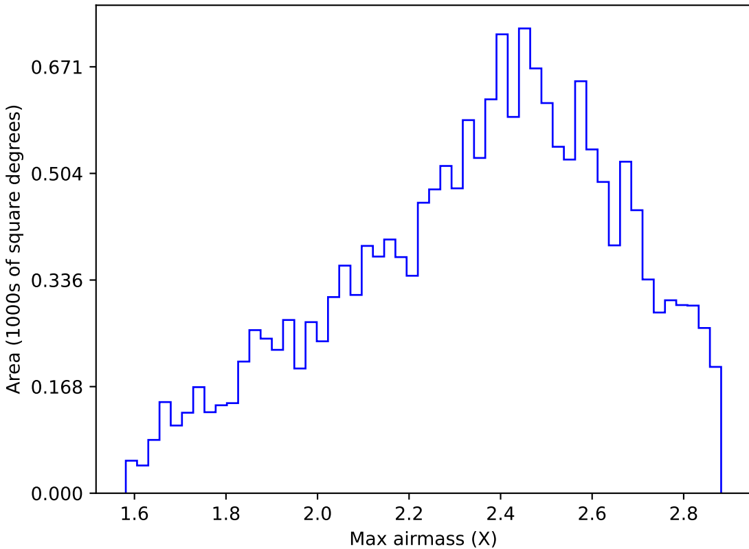
weather_cloudso20v3.4_10yrs WFD y band: Max airmass
