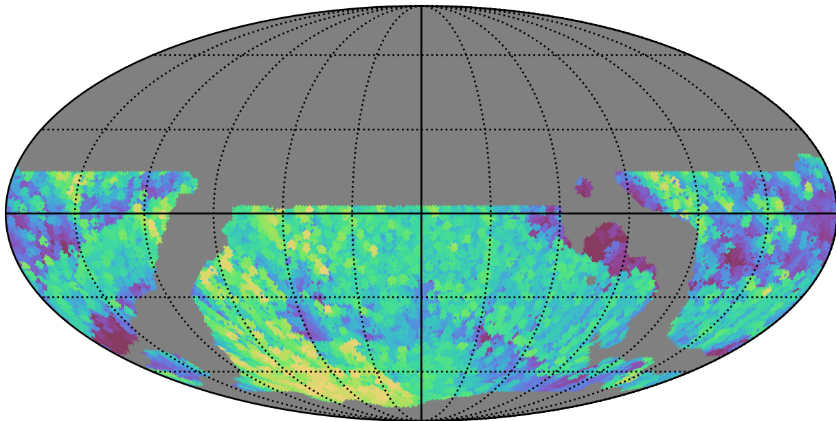
weather_cloudso20v3.4_10yrs WFD r band: Max airmass
