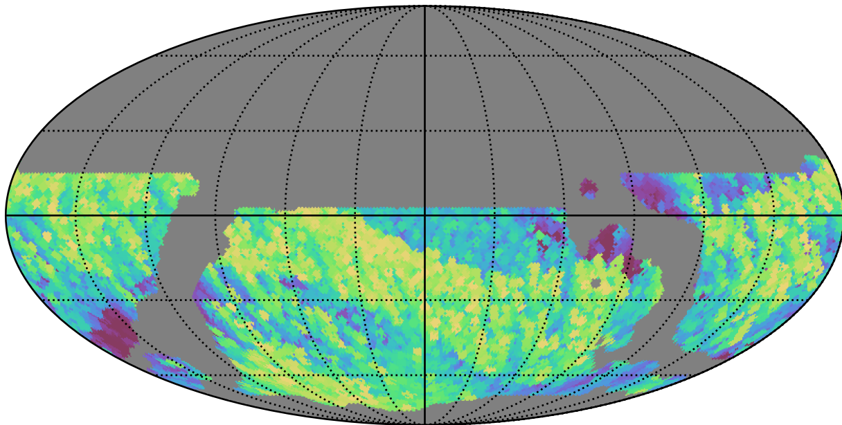
weather_cloudso20v3.4_10yrs WFD i band: Max airmass
