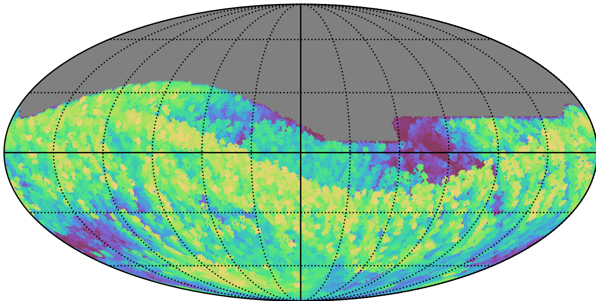
weather_cloudso20v3.4_10yrs All sky z band: Max airmass
