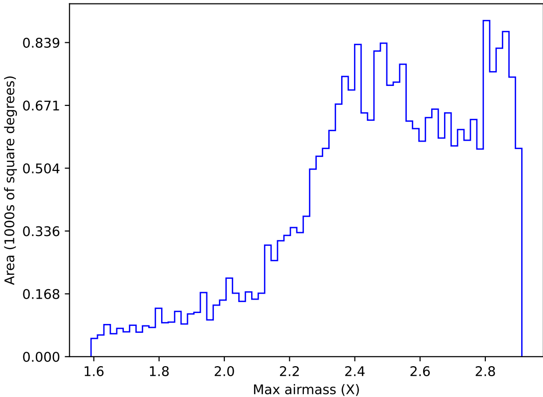
weather_cloudso20v3.4_10yrs All sky z band: Max airmass
