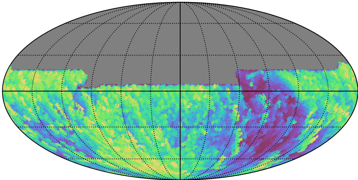
weather_cloudso20v3.4_10yrs All sky y band: Max airmass
