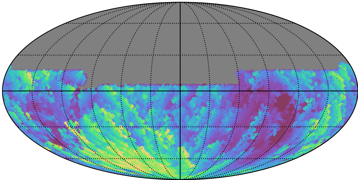
weather_cloudso20v3.4_10yrs All sky u band: Max airmass
