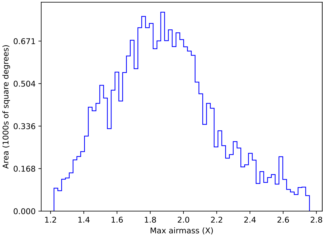
weather_cloudso20v3.4_10yrs All sky u band: Max airmass
