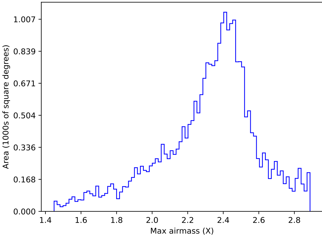
weather_cloudso20v3.4_10yrs All sky r band: Max airmass
