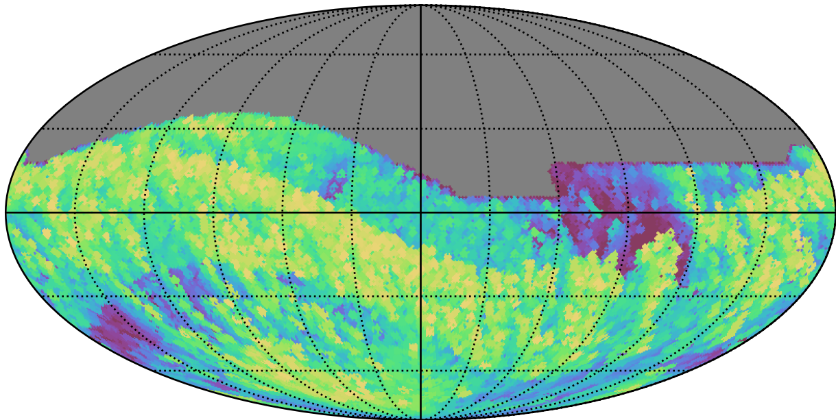
weather_cloudso20v3.4_10yrs All sky i band: Max airmass
