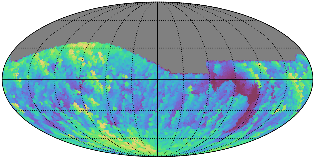
weather_cloudso20v3.4_10yrs All sky g band: Max airmass
