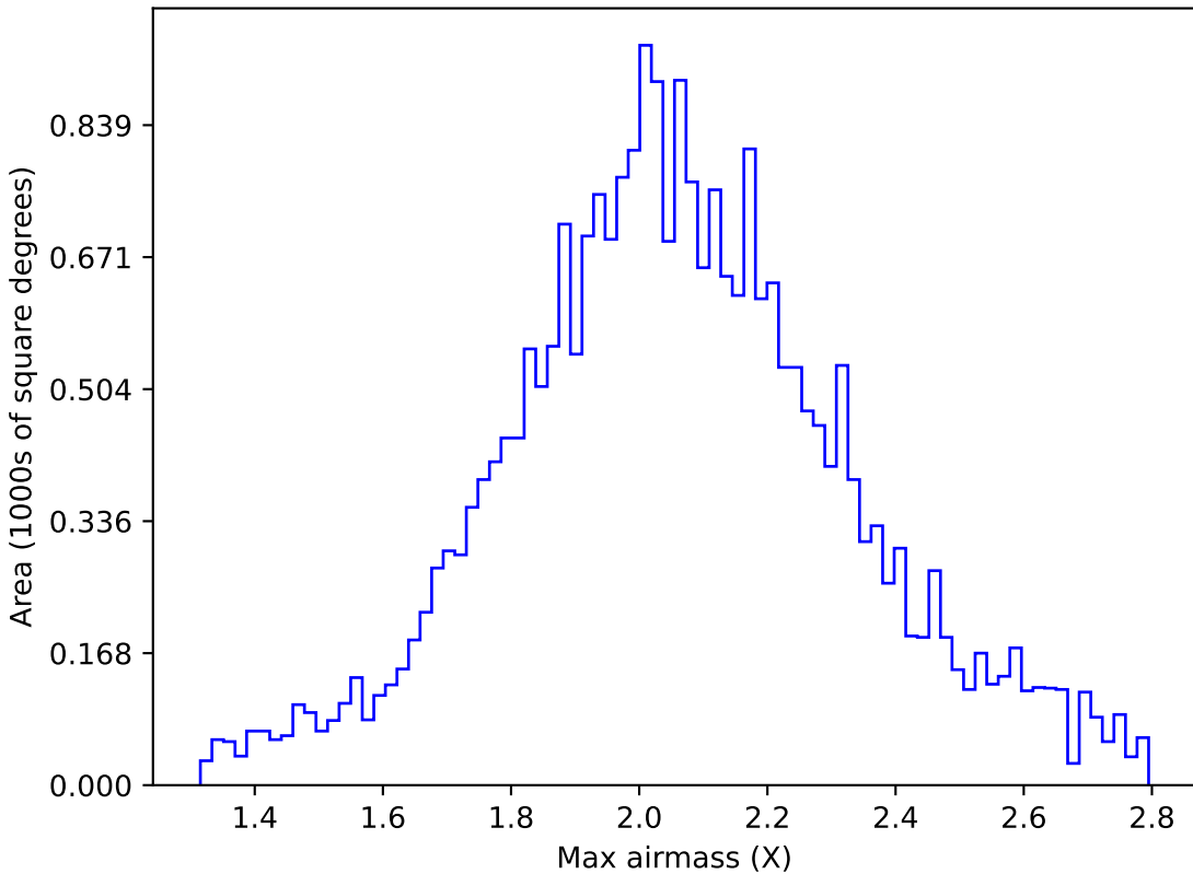
weather_cloudso20v3.4_10yrs All sky g band: Max airmass
