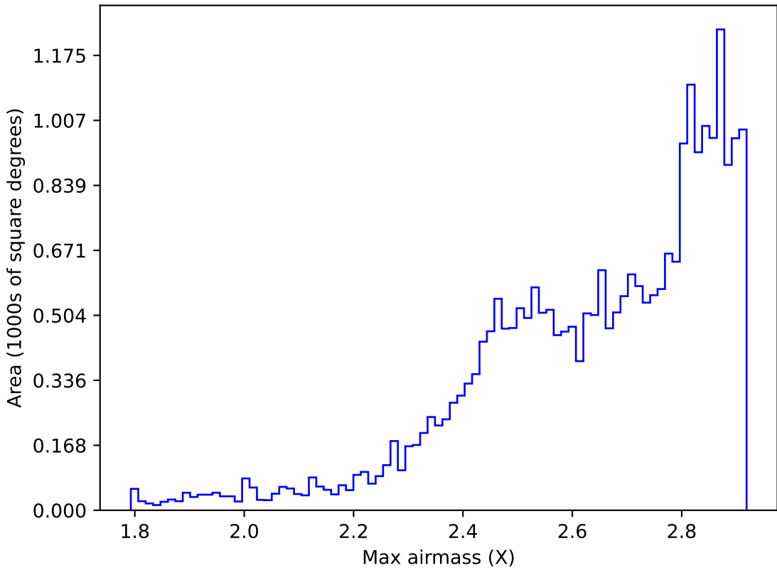
weather_cloudso20v3.4_10yrs All sky all bands: Max airmass
