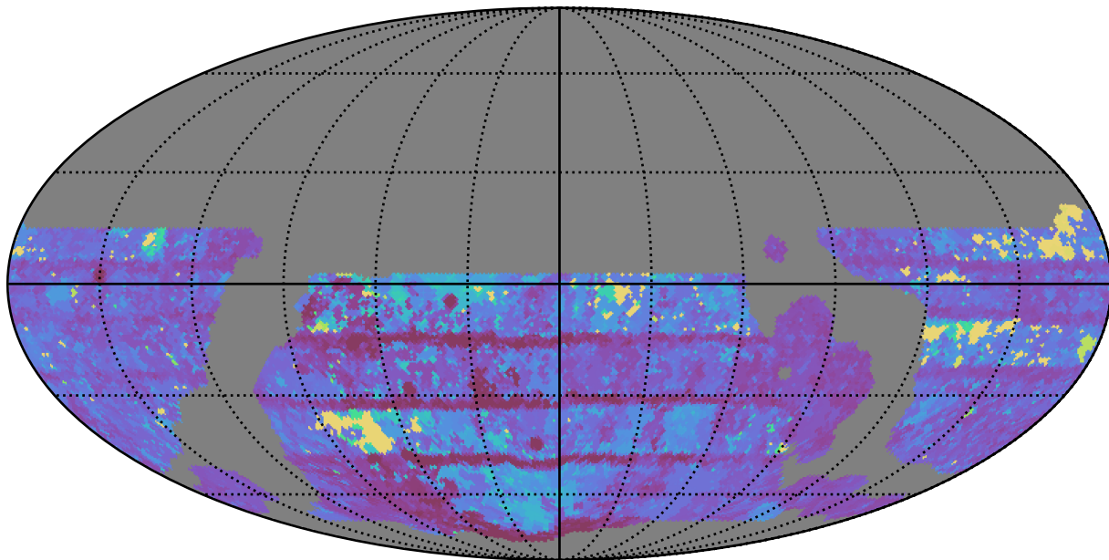
weather_cloudso20v3.4_10yrs WFD z band: Max Inter-Night Gap
