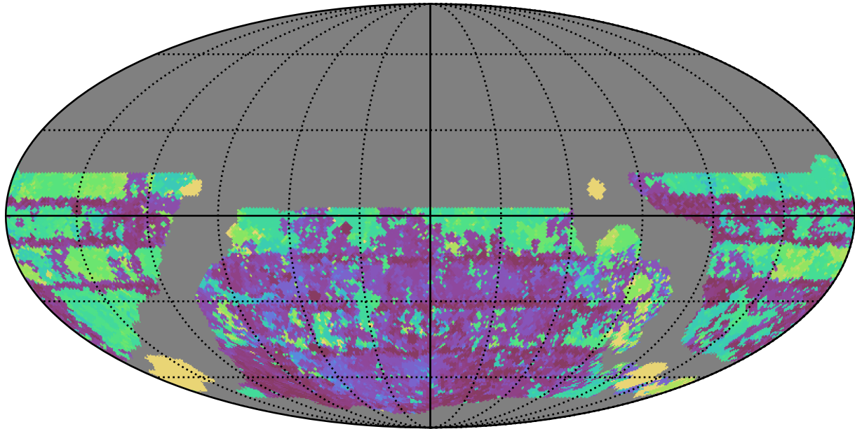
weather_cloudso20v3.4_10yrs WFD u band: Max Inter-Night Gap
