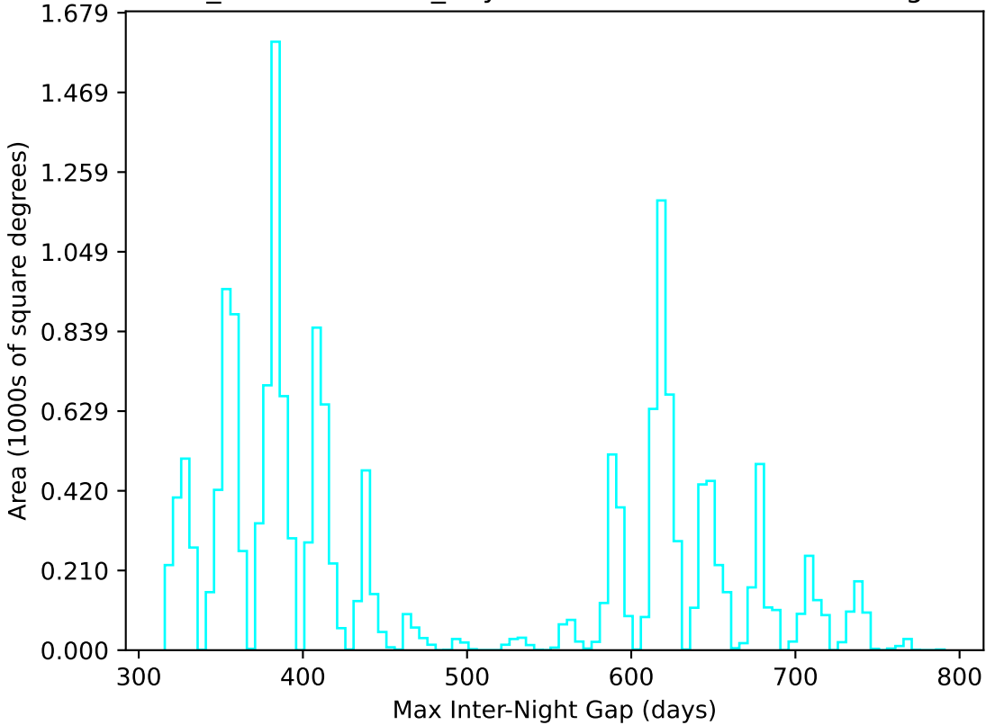
weather_cloudso20v3.4_10yrs WFD u band: Max Inter-Night Gap
