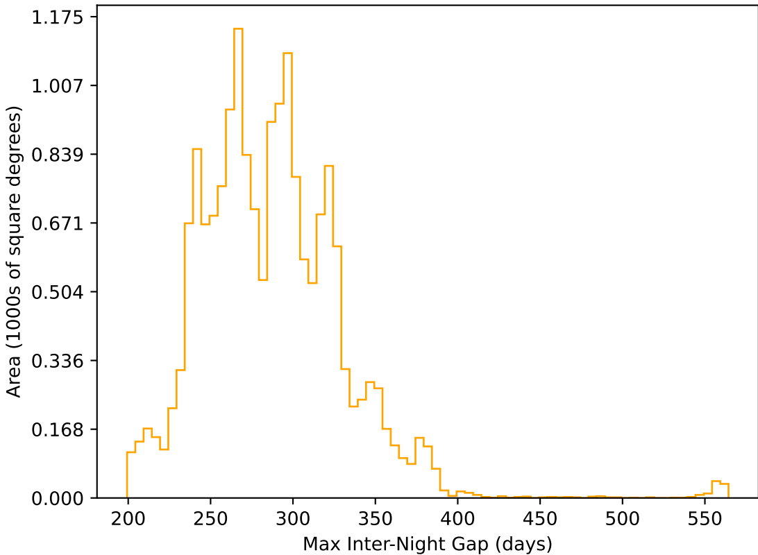
weather_cloudso20v3.4_10yrs WFD r band: Max Inter-Night Gap
