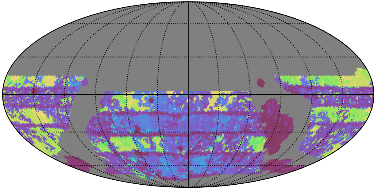
weather_cloudso20v3.4_10yrs WFD g band: Max Inter-Night Gap
