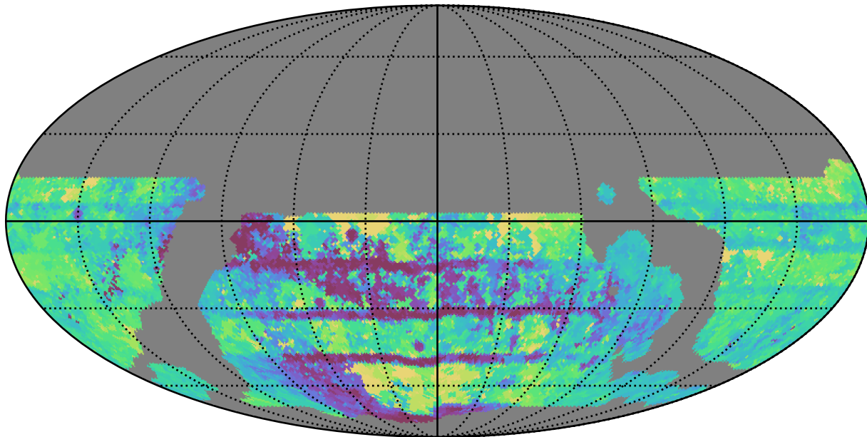
weather_cloudso20v3.4_10yrs WFD all bands: Max Inter-Night Gap
