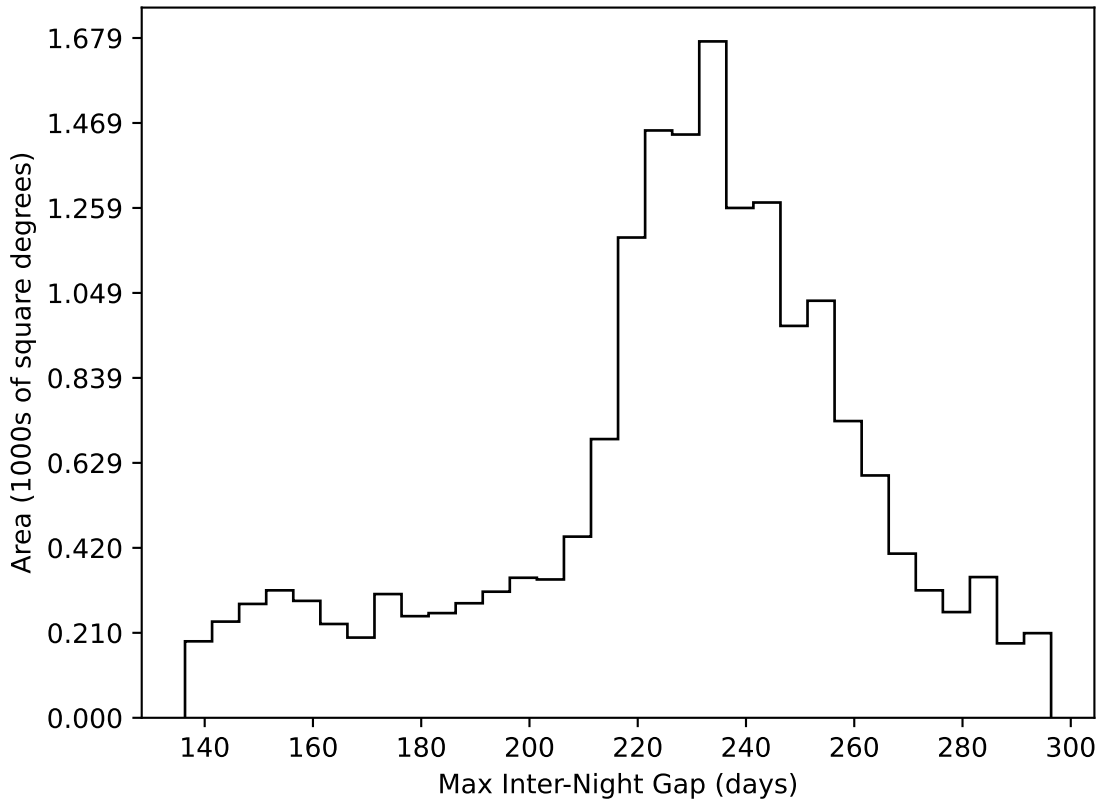
weather_cloudso20v3.4_10yrs WFD all bands: Max Inter-Night Gap
