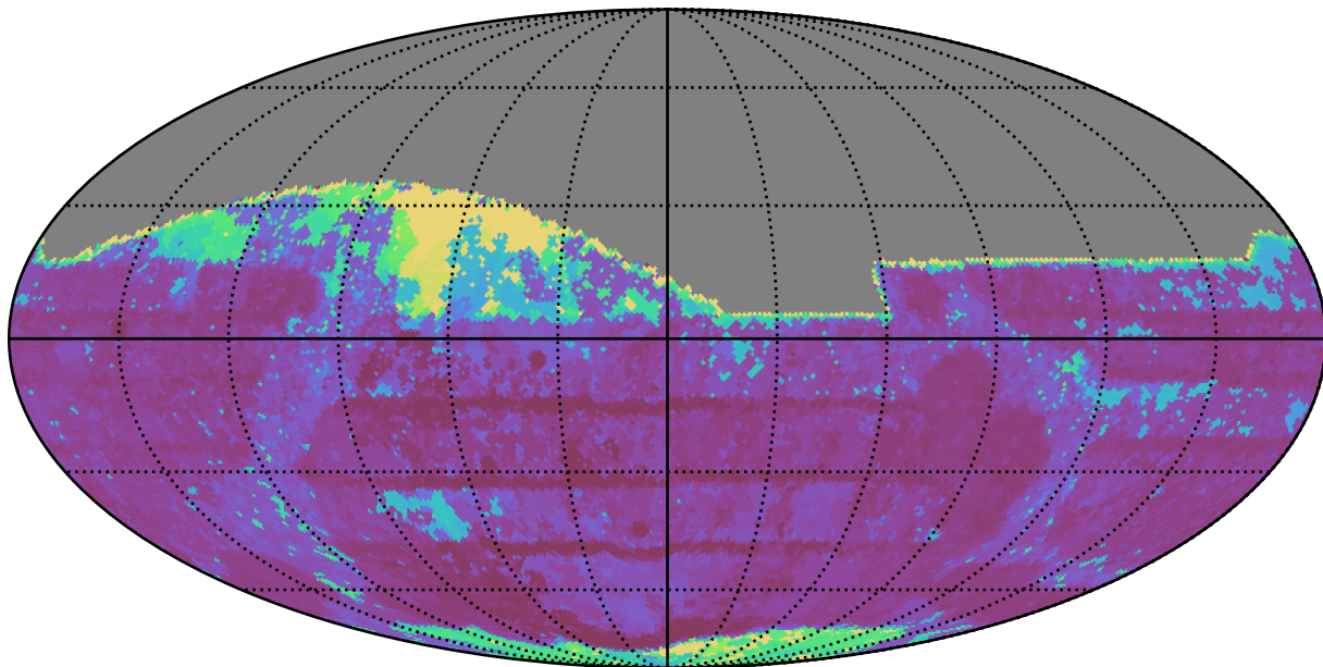
weather_cloudso20v3.4_10yrs All sky z band: Max Inter-Night Gap
