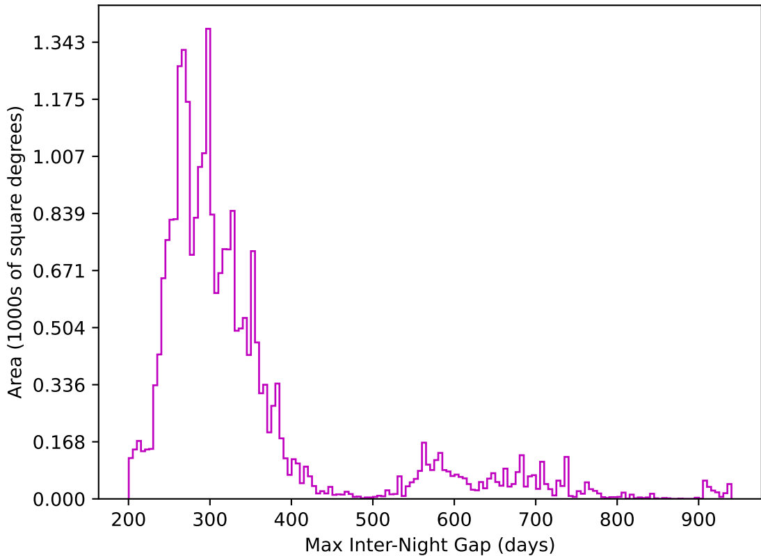
weather_cloudso20v3.4_10yrs All sky z band: Max Inter-Night Gap
