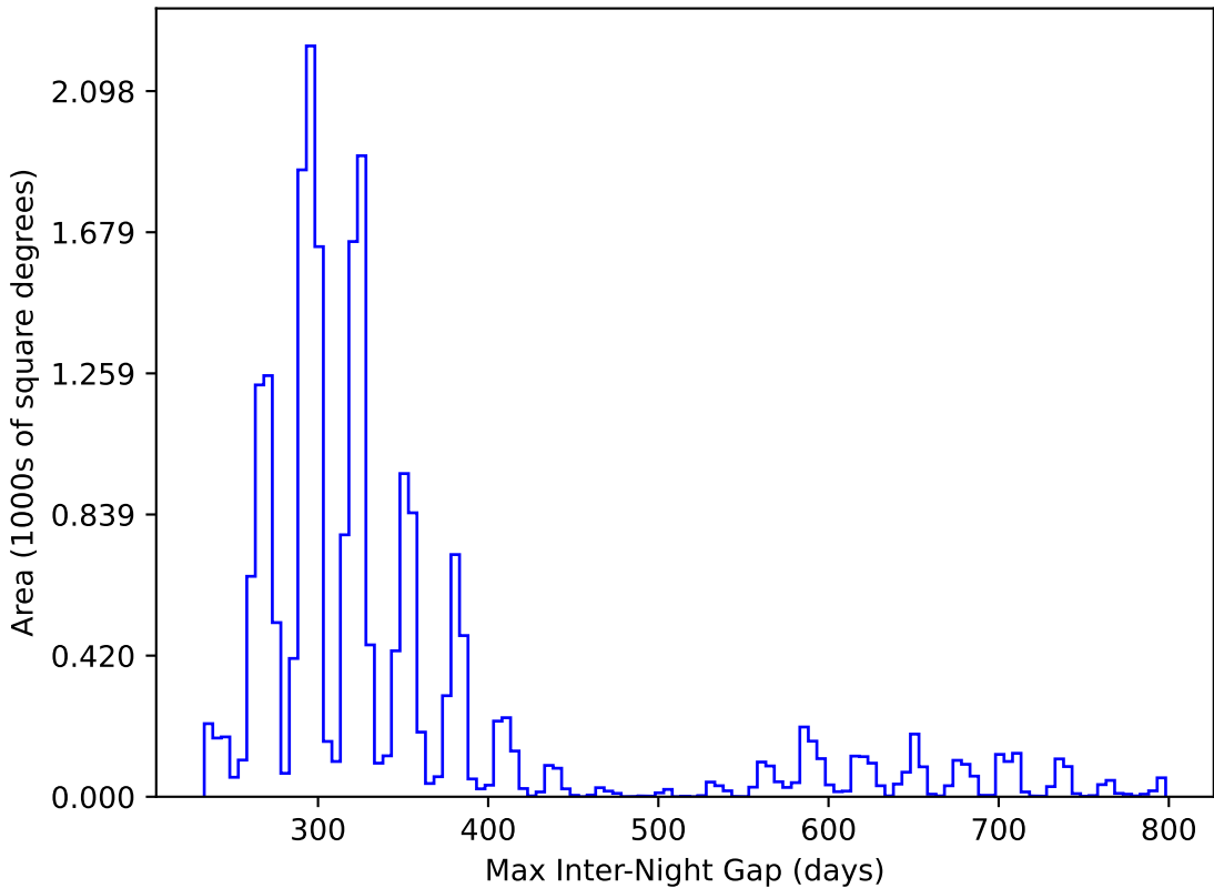
weather_cloudso20v3.4_10yrs All sky y band: Max Inter-Night Gap
