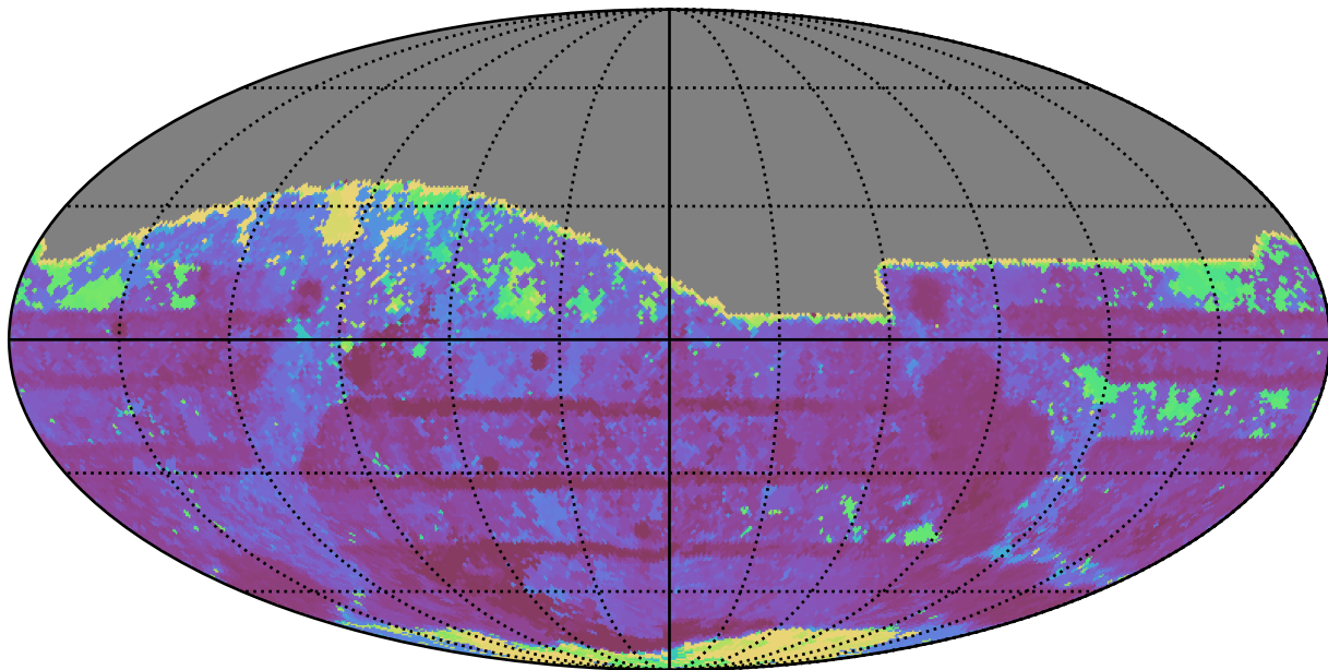
weather_cloudso20v3.4_10yrs All sky r band: Max Inter-Night Gap
