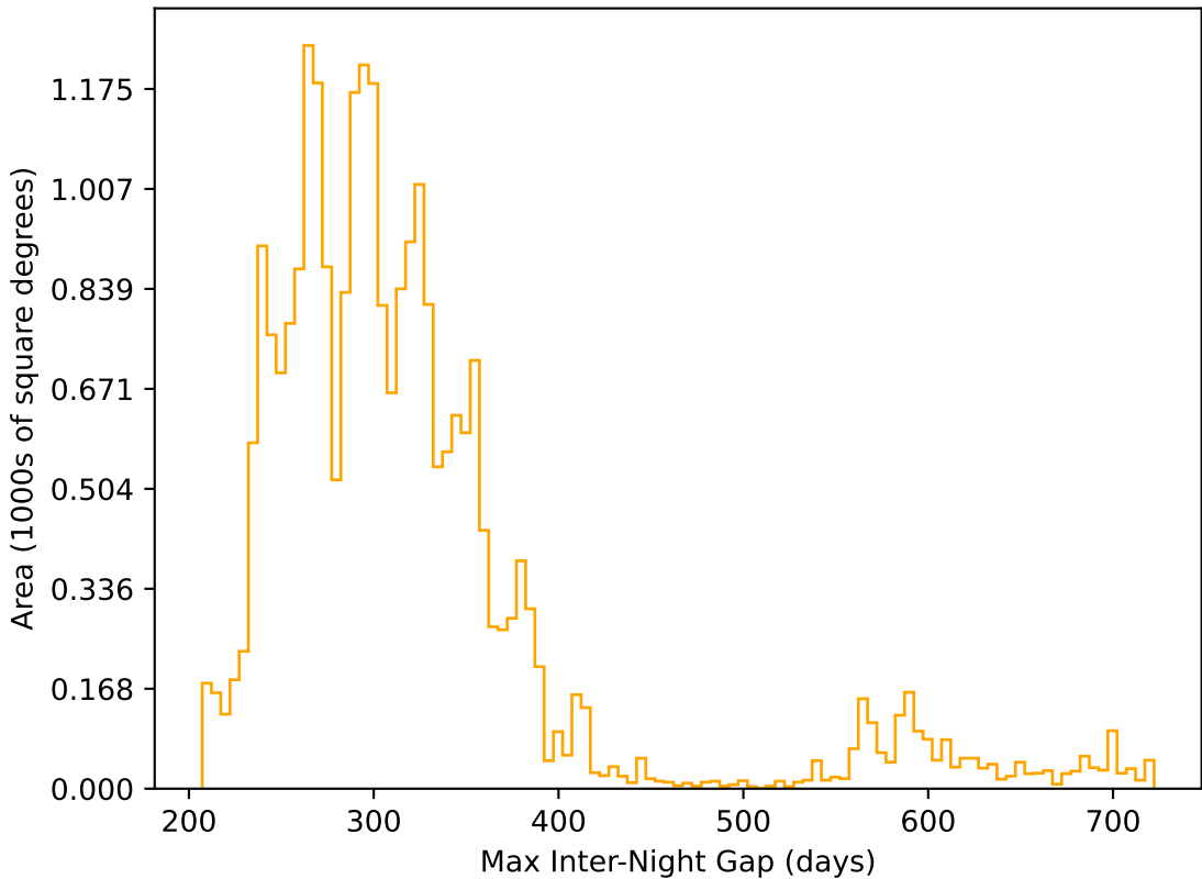
weather_cloudso20v3.4_10yrs All sky r band: Max Inter-Night Gap
