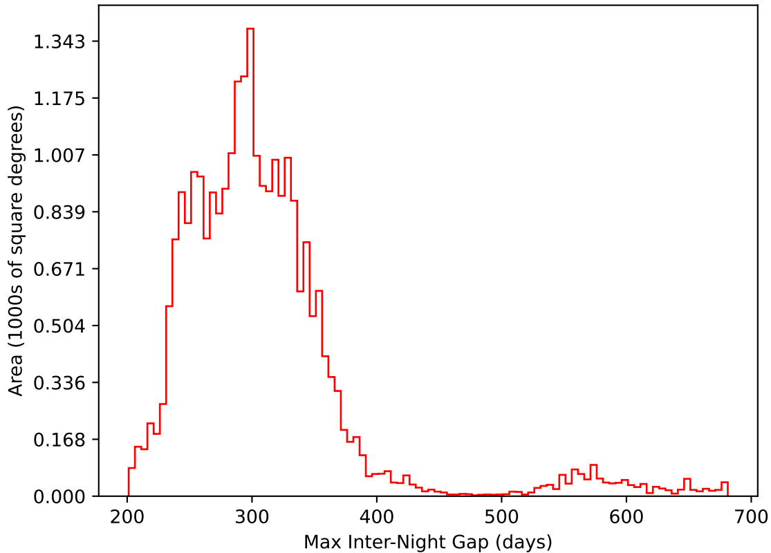
weather_cloudso20v3.4_10yrs All sky i band: Max Inter-Night Gap
