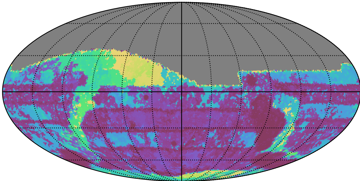
weather_cloudso20v3.4_10yrs All sky g band: Max Inter-Night Gap
