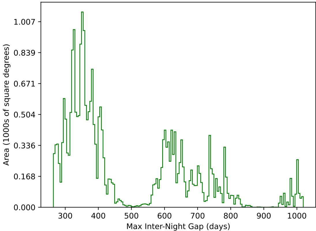
weather_cloudso20v3.4_10yrs All sky g band: Max Inter-Night Gap
