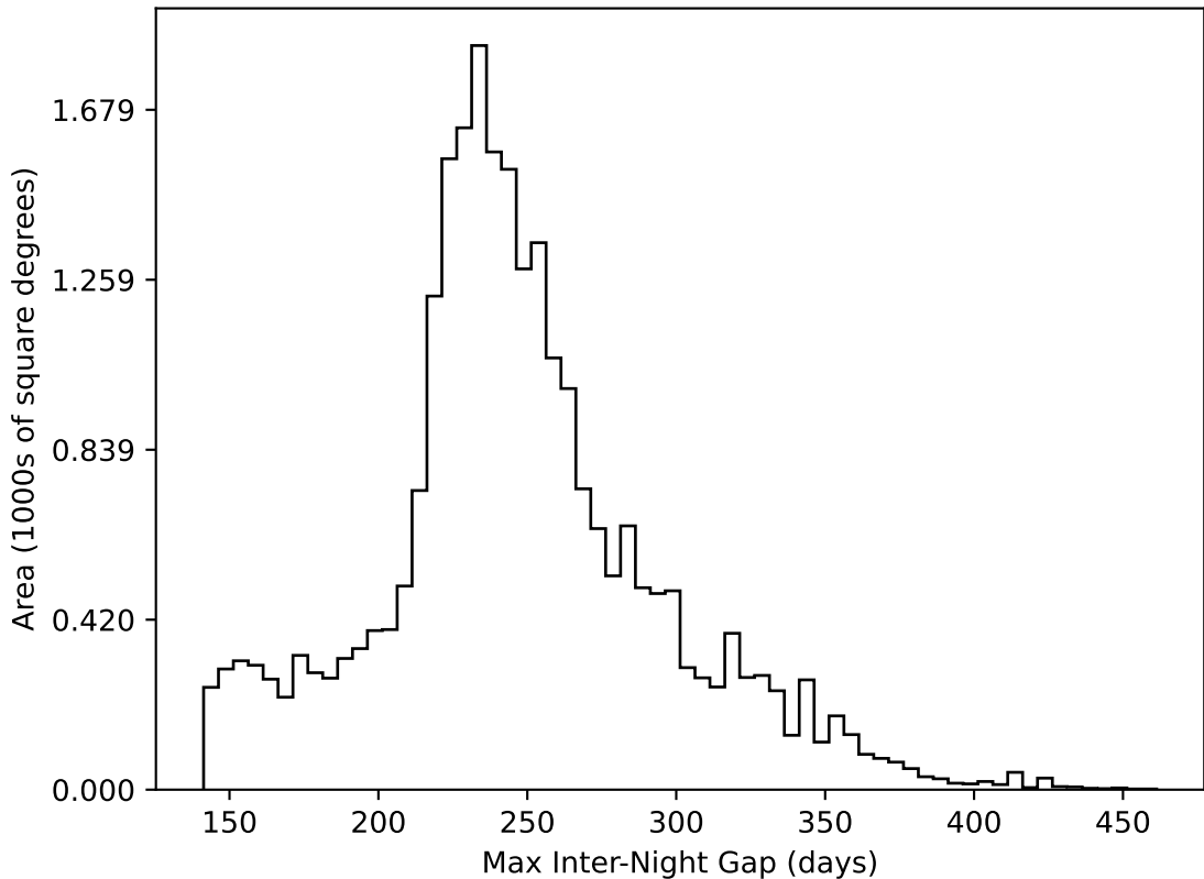
weather_cloudso20v3.4_10yrs All sky all bands: Max Inter-Night Gap
