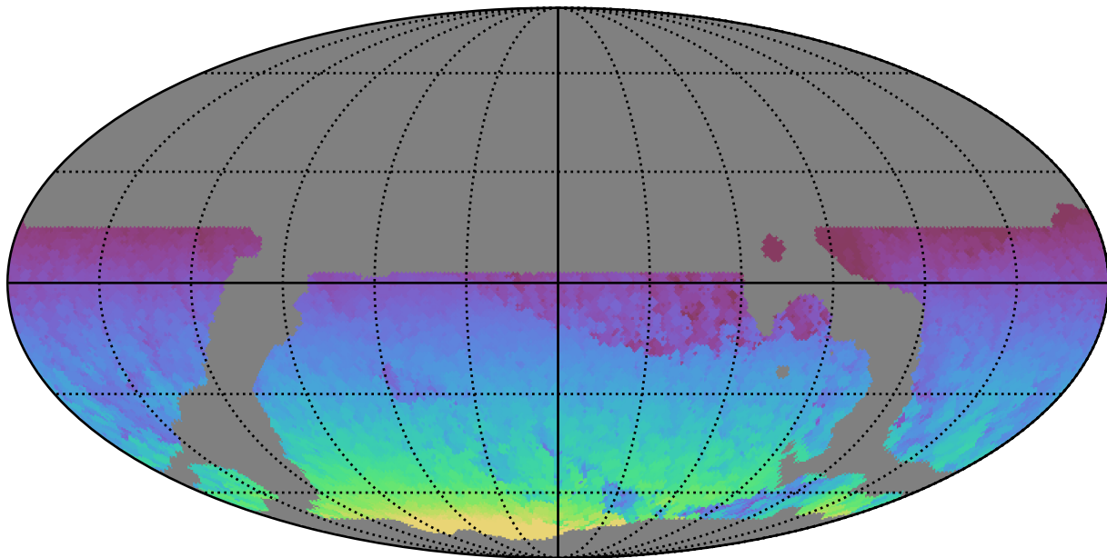
weather_cloudso20v3.4_10yrs WFD all bands: Max HA
