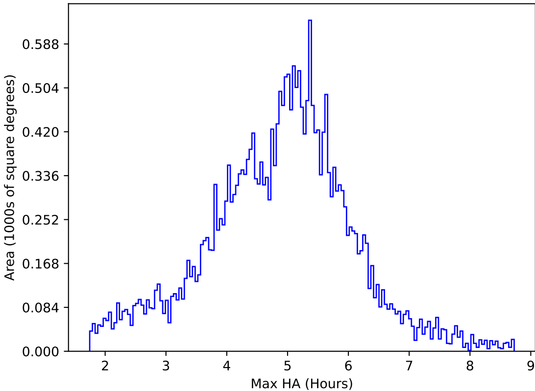
weather_cloudso20v3.4_10yrs All sky all bands: Max HA
