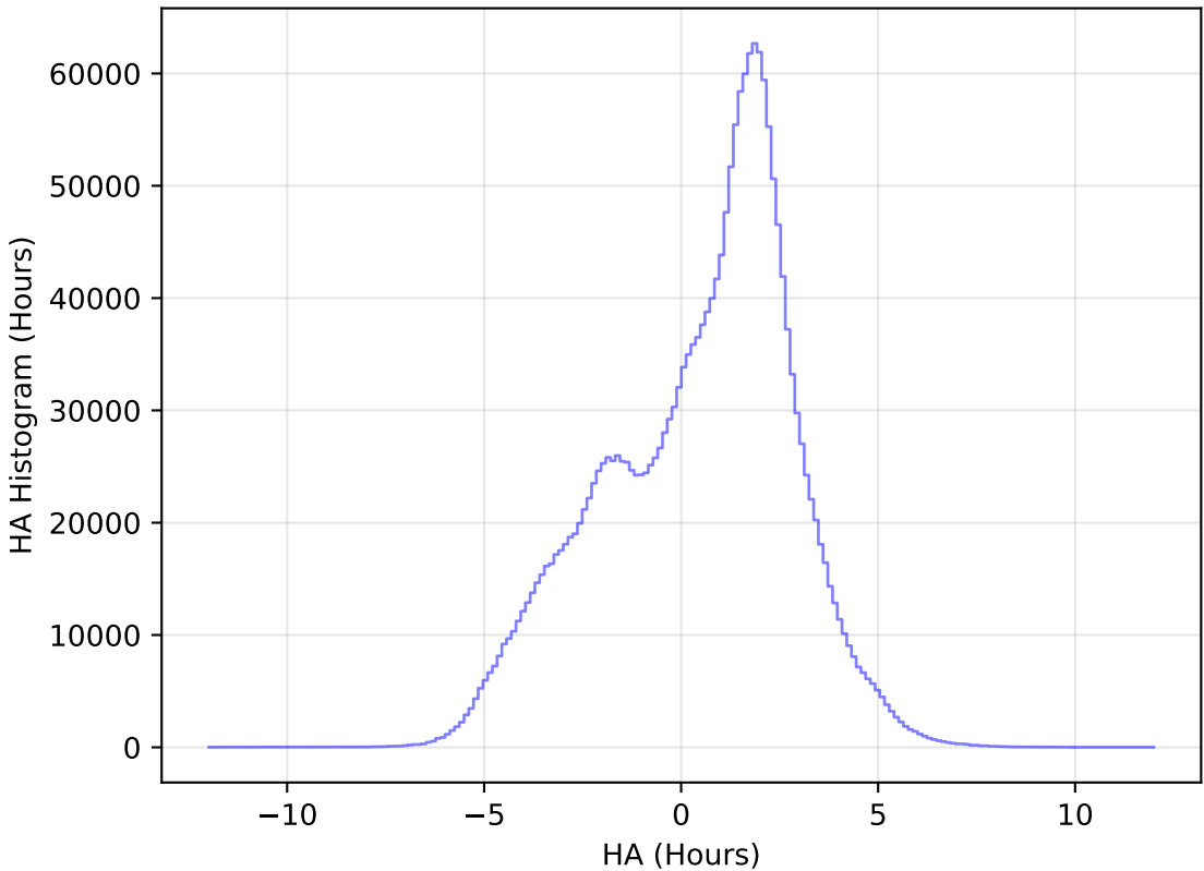
weather_cloudso20v3.4_10yrs WFD all bands: HA Histogram
