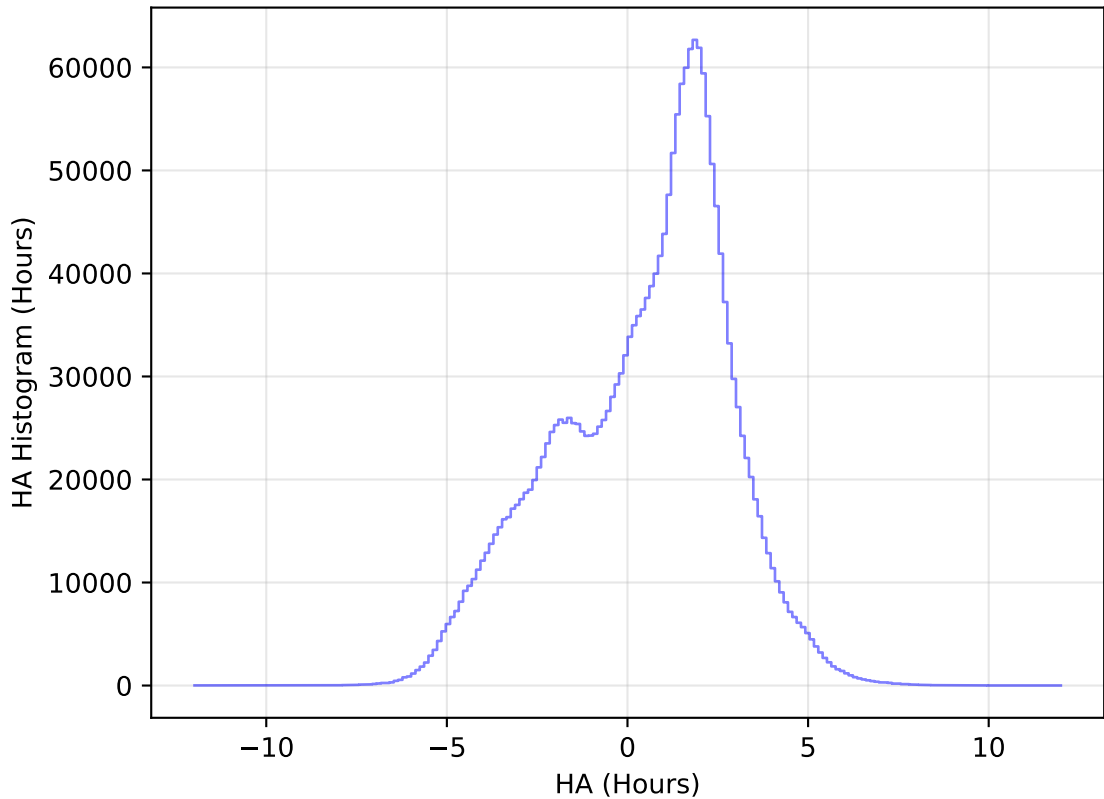
weather_cloudso20v3.4_10yrs All sky all bands: HA Histogram
