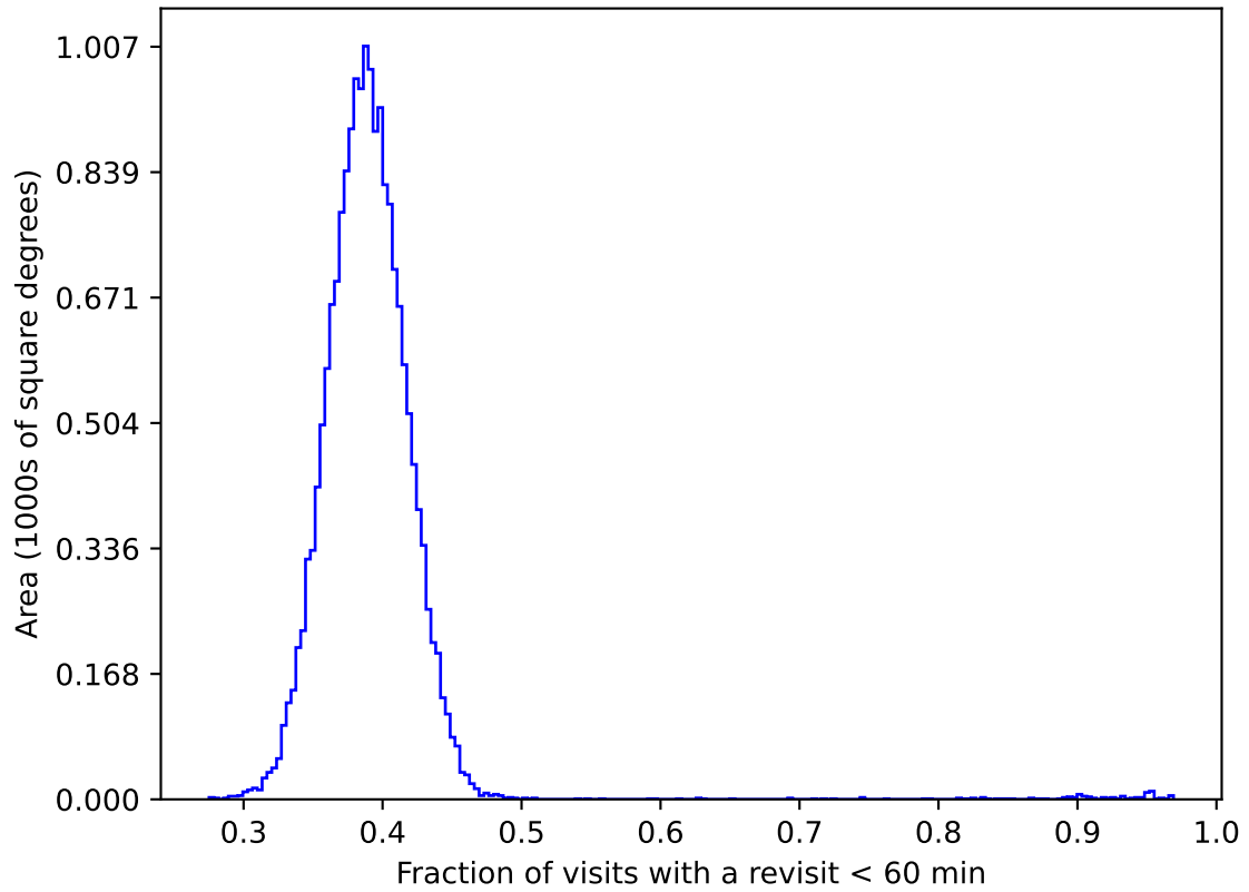
weather_cloudso20v3.4_10yrs gri WFD: Fraction of visits with a revisit < 60 min
