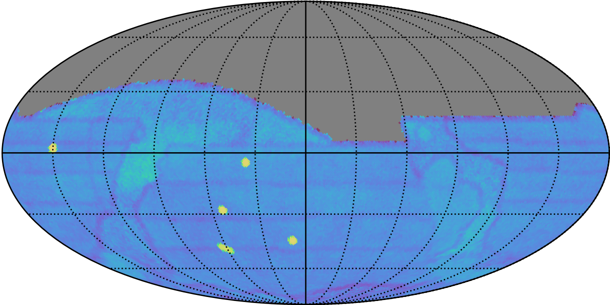
weather_cloudso20v3.4_10yrs gri All sky: Fraction of visits with a revisit < 60 min
